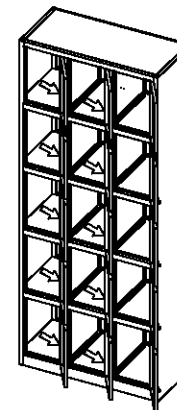
5 Install the division plates. (Pay attention to the difference of upper and lower ones, the upper one is small and lower one is big.)
