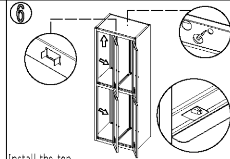
6 Install the top plate, and then install the upper and lower division plates as shown in the picture.
