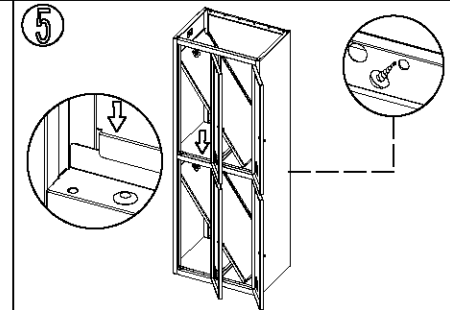
5 Install the middle plate firstly, and put the upper division plate into the locker.
