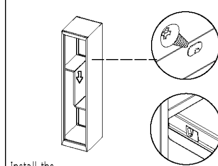
6 Install the division plate as shown in the picture.
